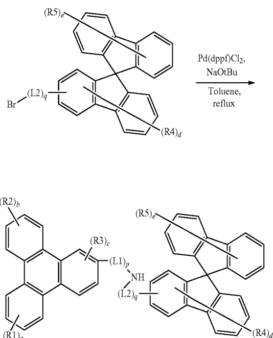
[Reaction Formula 2-2]
