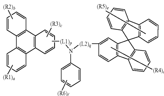
[Chemical Formula 4]
