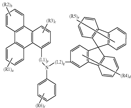
[Chemical Formula 12]
