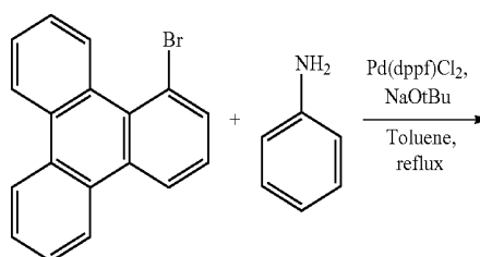
[Reaction Formula 3-2]
