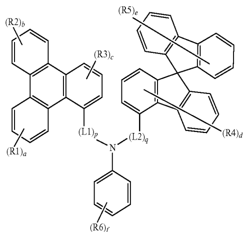
[Chemical Formula 12]
