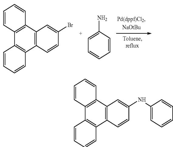
[Reaction Formula 3-1]
