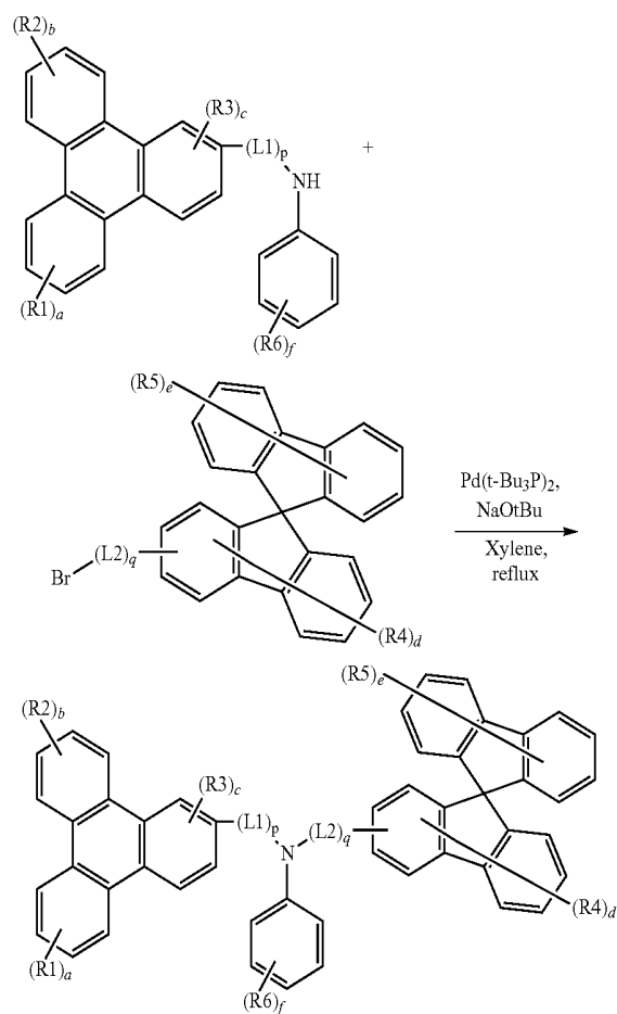
[Reaction Formula 1-2]
