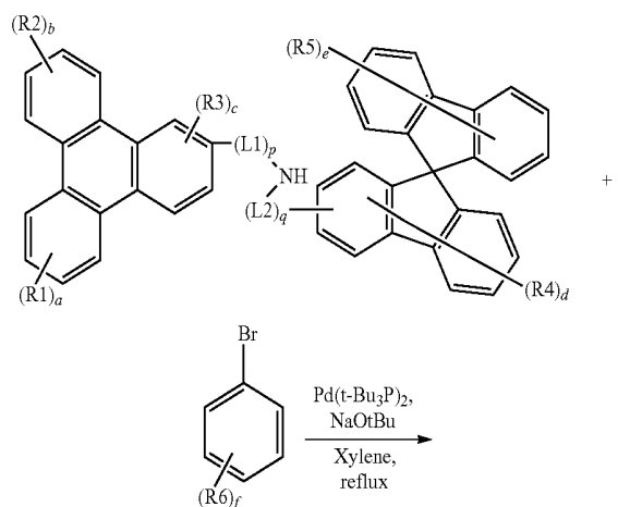
[Reaction Formula 2-2]
