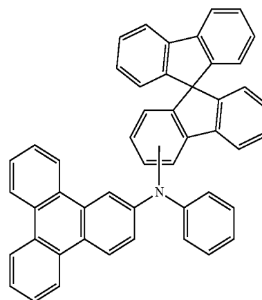
[Reaction Formula 3-2]
