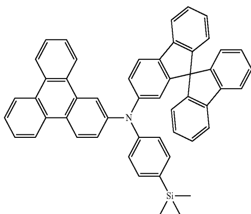
[Compound 1-4]
