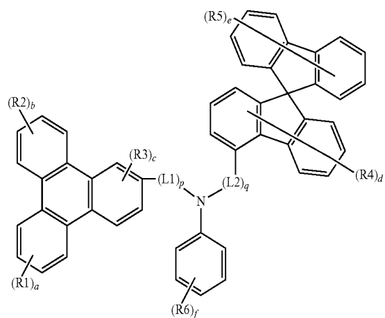
[Chemical Formula 9]
