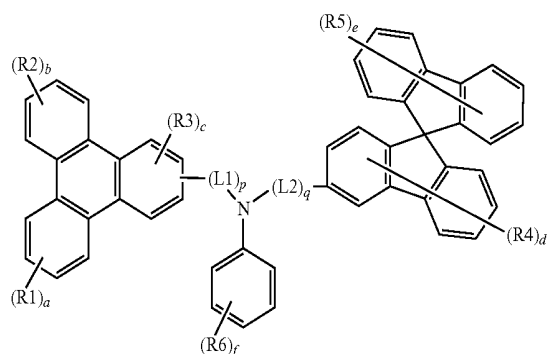
[Chemical Formula 5]
