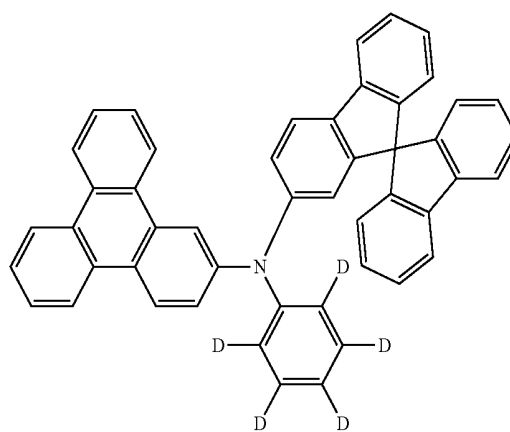
[Compound 1-5]
