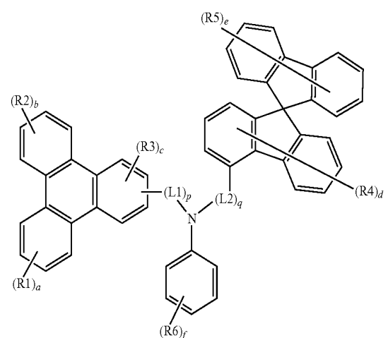
[Chemical Formula 6]
