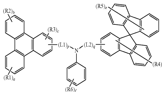
[Chemical Formula 1]
