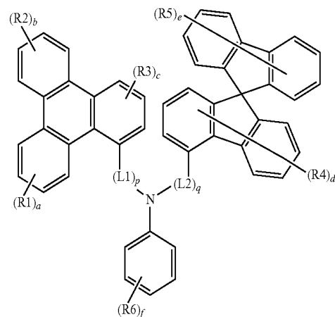
[Chemical Formula 12]
