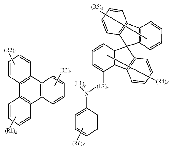
[Chemical Formula 9]
