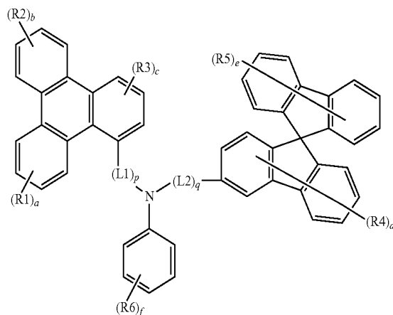
[Chemical Formula 12]
