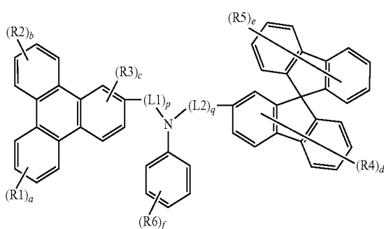
[Chemical Formula 7]
