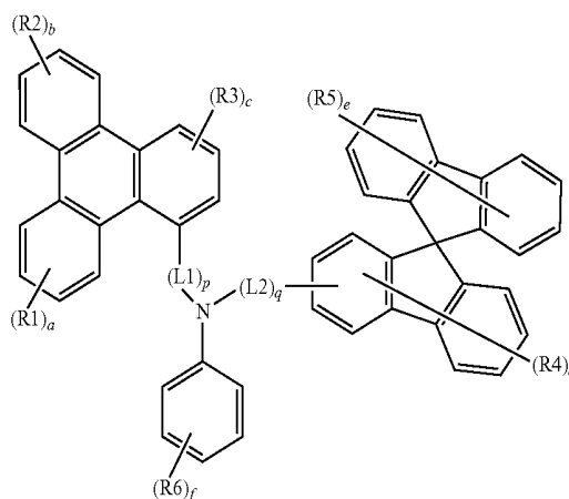
[Chemical Formula 3]
