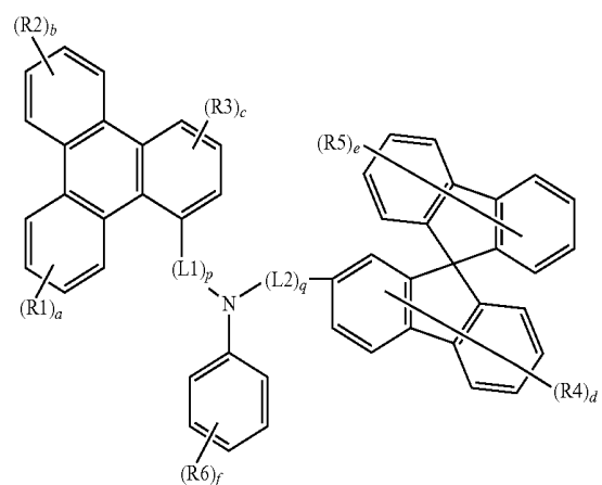
[Chemical Formula 10]
