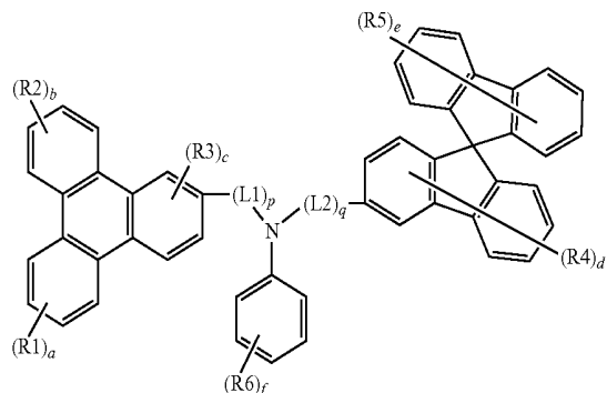
[Chemical Formula 9]
