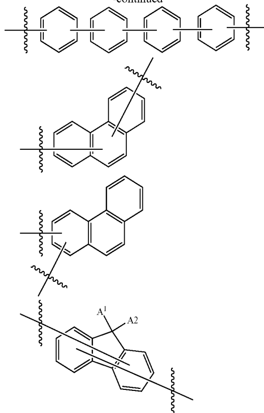
[Chemical Formula 11]
