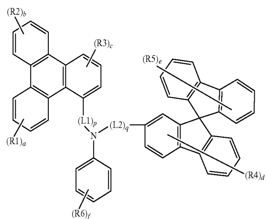
[Chemical Formula 10]
