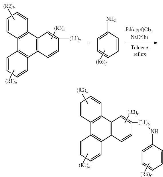
[Reaction Formula 1-2]
