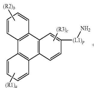
[Reaction Formula 2-1]
